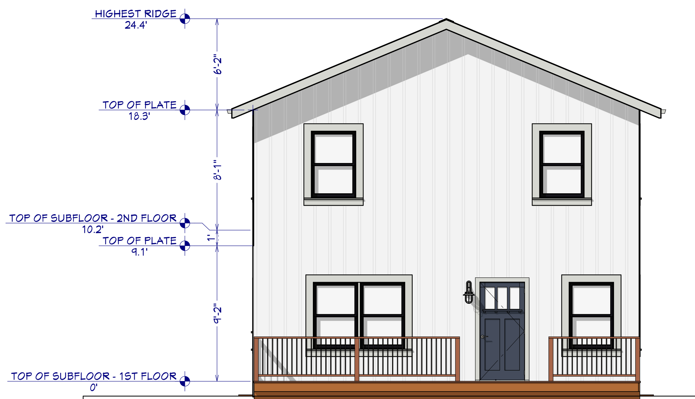
2 REAR ELEVATION 1/4"=1'-0"
