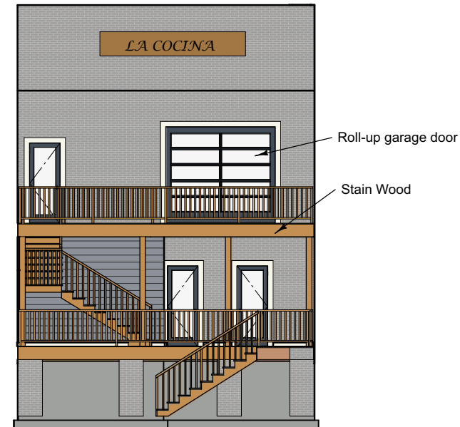
④ Rear Elevation Details 1/8"=1'-0"
